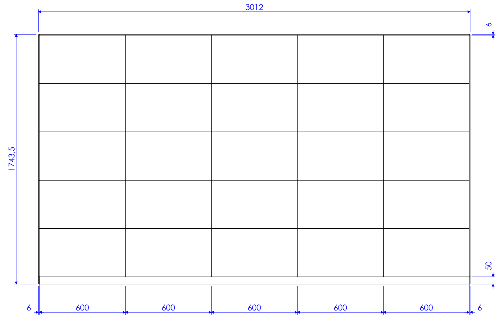
FRONT VIEW
