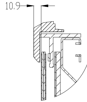
Section A-A Scale 2/1
