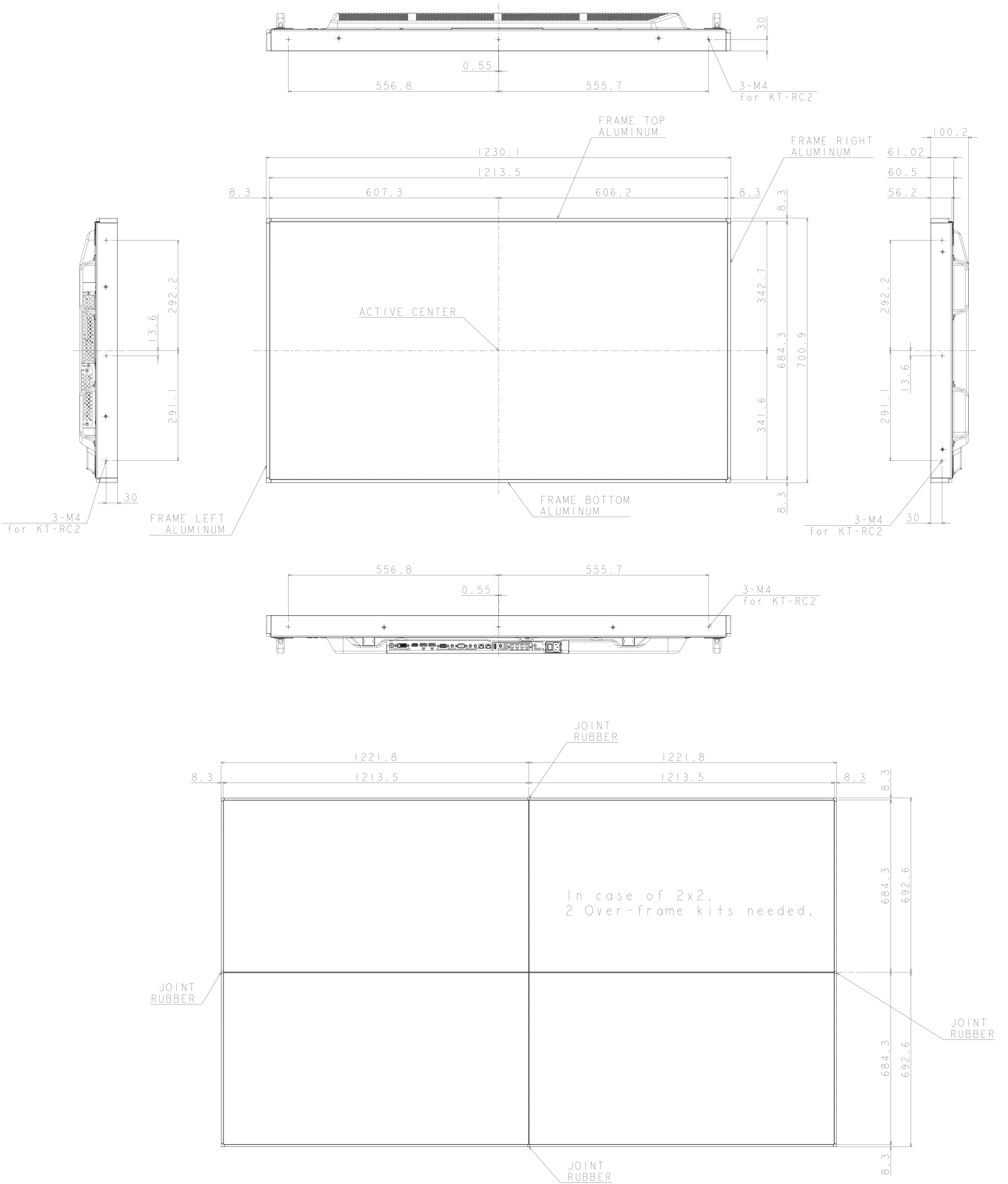
X554UN with KT-55UN-OF2 OUTLINE DRAWING
