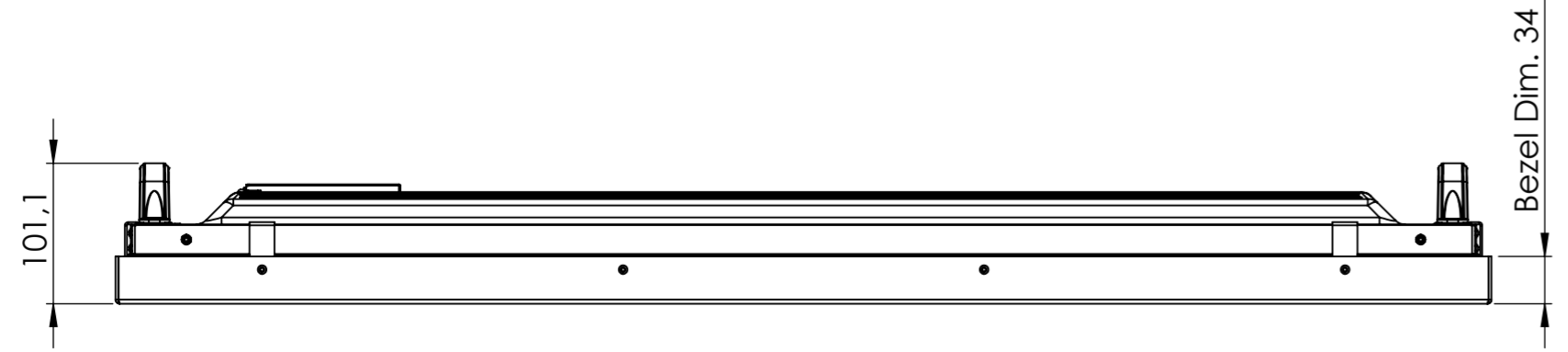
Top View
