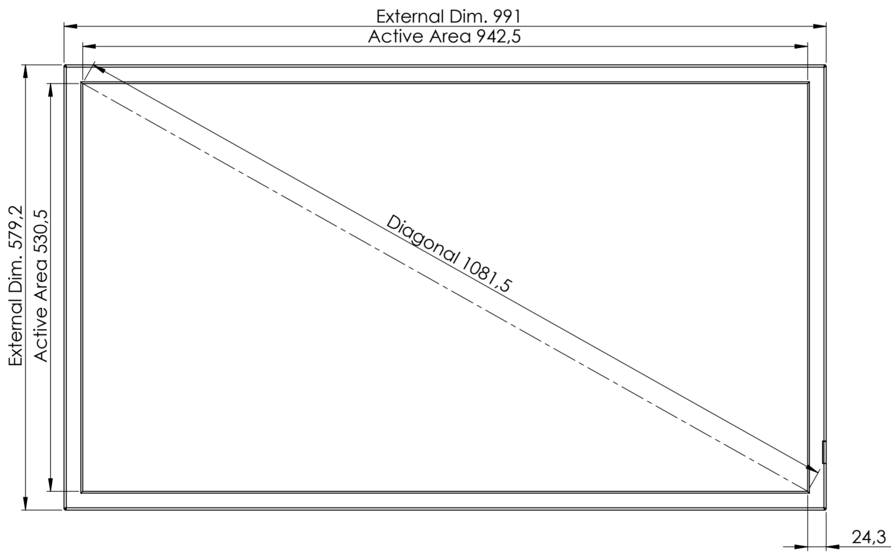
Front View
